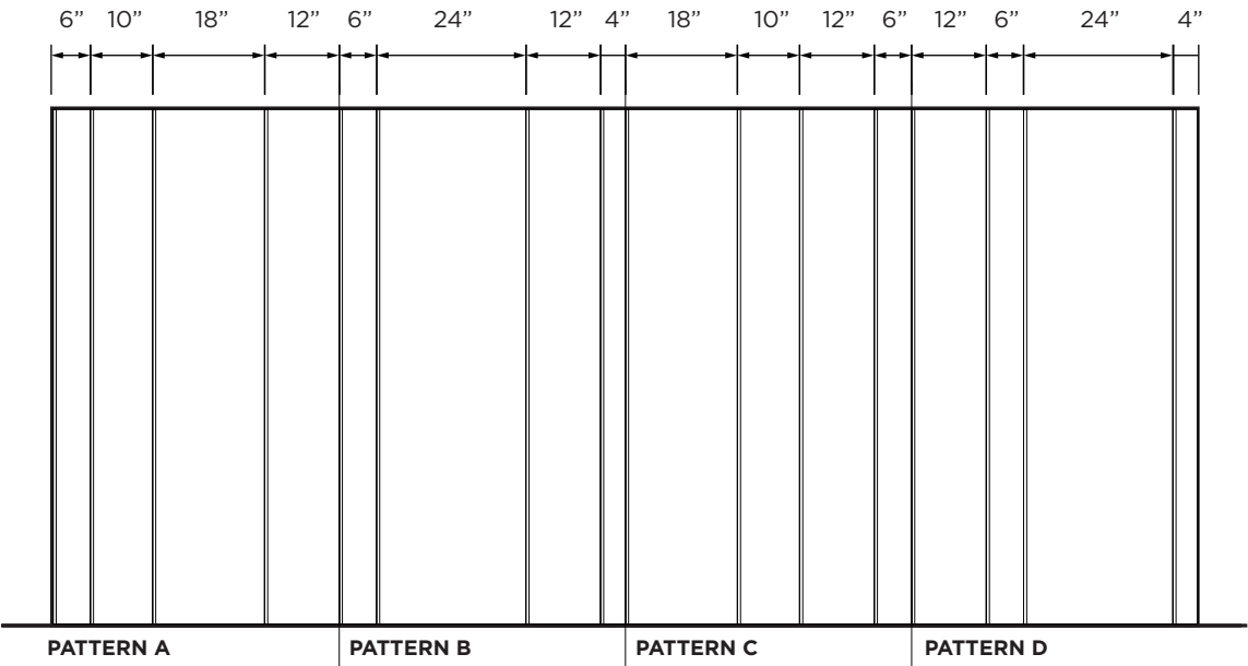
PATTERN LAYOUT SEQUENCE
