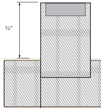
SECTION DETAIL | WOOD BARS WITH STRIP
