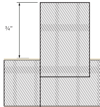
SECTION DETAIL | SOLID WOOD BARS
