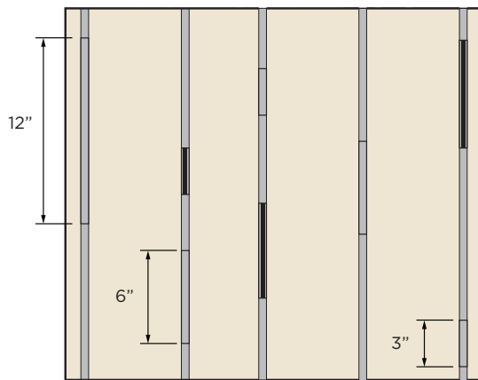
PATTERN LAYOUT DETAIL | WITH SOLID WOOD BARS OR WITH STRIP
